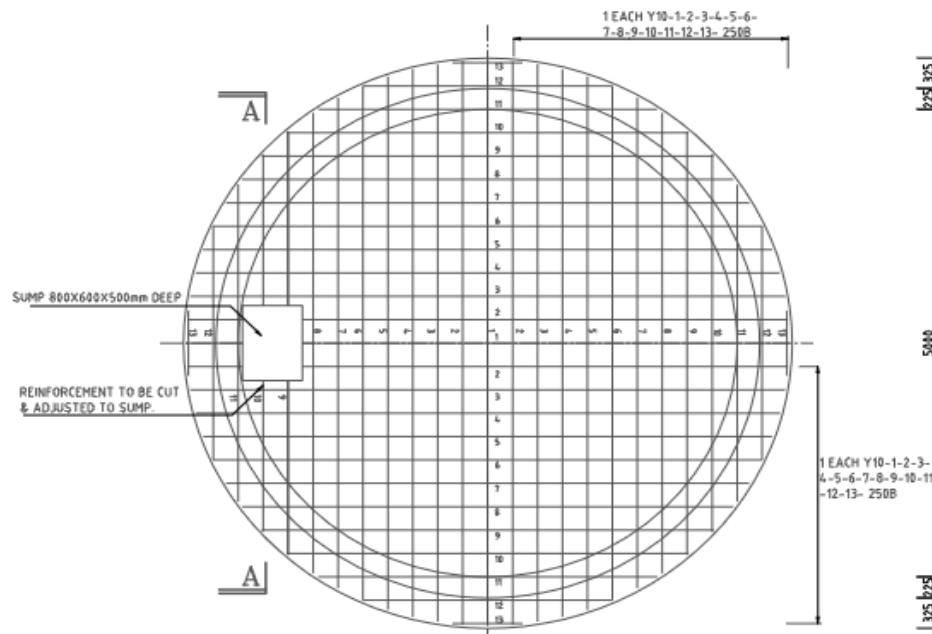
BOTTOM REINFORCEMENT OF FLOOR SLAB SCALE 1:50
