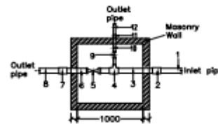
MASONRY CHAMBER PLAN
