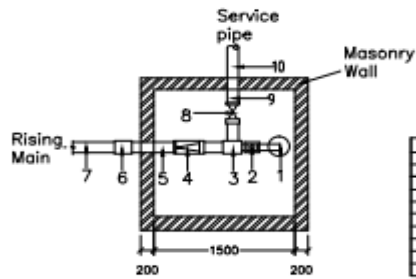
BOREHOLE CHAMBER PLAN
