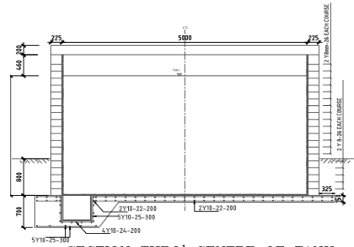
SECTION THRO' CENTRE OF TANK SCALE 1:50
